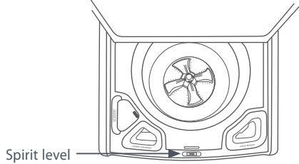
Fig.10 Leveling – Step 7
